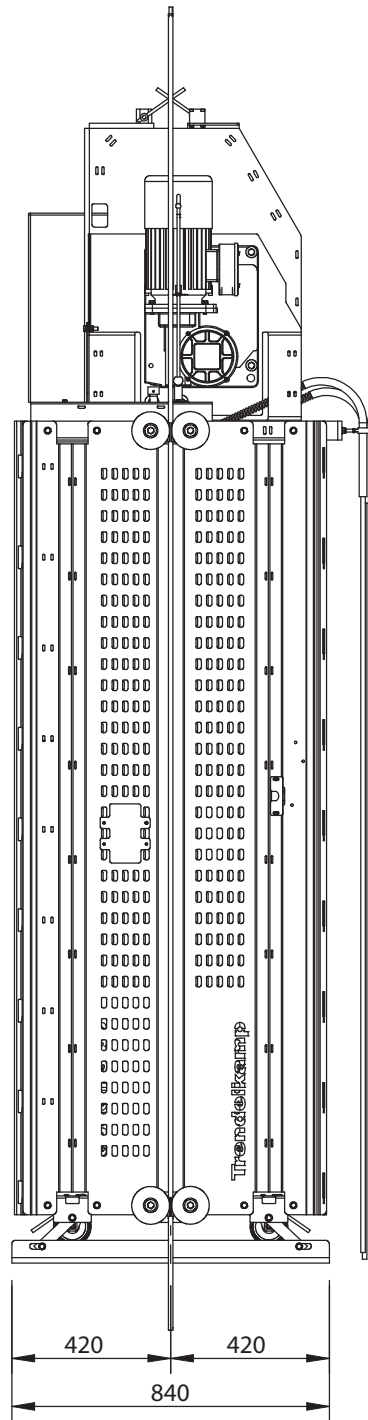
Side View
