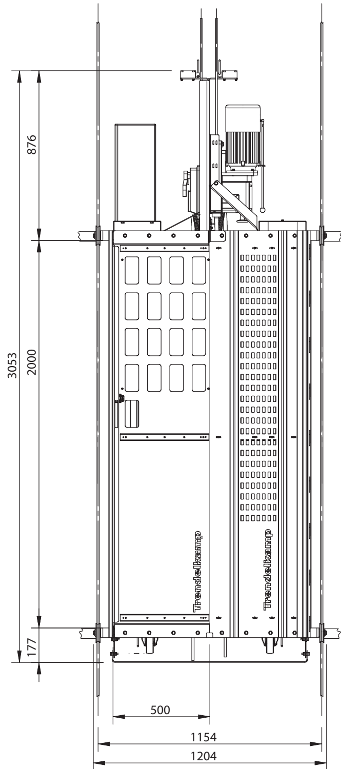
Front View
